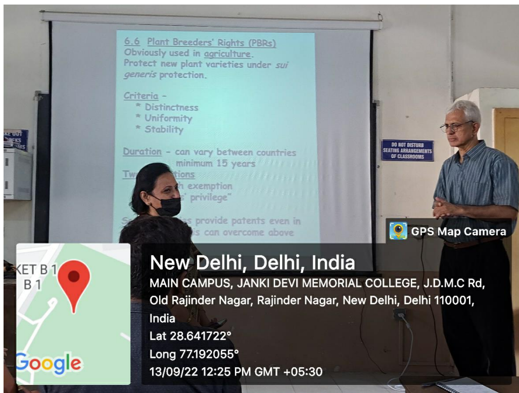
Figure 1: Access-Innovation Trade-Off
