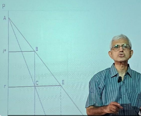
Figure 1: Access-Innovation Trade-Off
